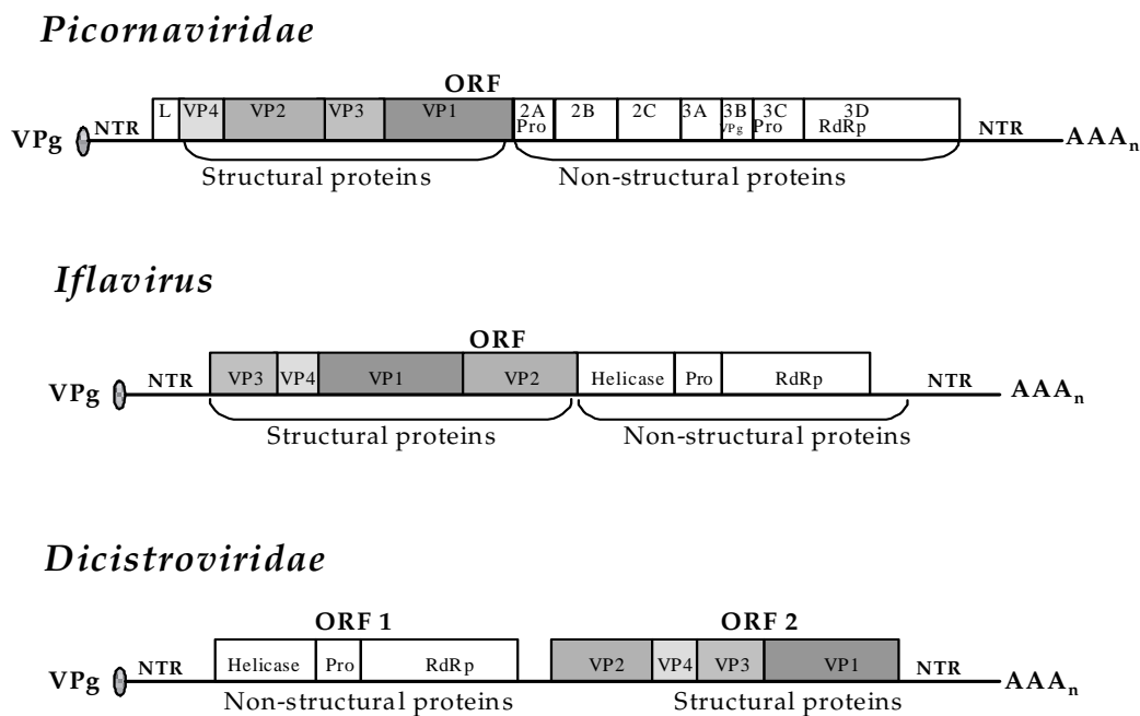
Figure 1-3: Schematic diagram of the genome organisation of Picornaviridae , Iflavirus and Dicistroviridae . The genome-linked protein (VPg) on the 5' end has been shown to be present in picorna-like viruses such as Cricket paralysis virus and Drosophila C virus (King & Moore, 1988). The structural proteins (VP1-VP4), shaded in the diagram, play a role in virus attachment to the host cell. Some picornaviruses (cardioviruses and aphthoviruses) encode a leader protein (L) at the beginning of the ORF. The 5' a nontranslated region (NTR) contains an internal ribosome entry site (IRES) in the three groups. Dicistroviridae have a second IRES in the intergenic region. The viruses belonging to these groups have a polyadenylated tail on the 3' end of the genome.
