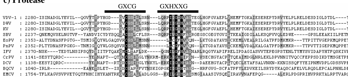
Figure 3-3: Multiple sequence alignment of VDV-1 with picorna-like viruses for (a) RdRp sequences (b) helicase and (c) protease domains. Conserved regions corresponding to those recognised by Koonin & Dolja (1993) are indicated with bars above the protein alignment. The black shading indicates 100% sequence identity and the dark grey shading indicates 80% identity. The light grey shading shows 60% identity. The numbers at the beginning of the sequences represent the amino acid position from the ORF start. The numbers within sequences represent the number of omitted amino acids. The amino acid sequences were deduced from nucleotide sequences for which accession numbers are given in Table 3-1.
